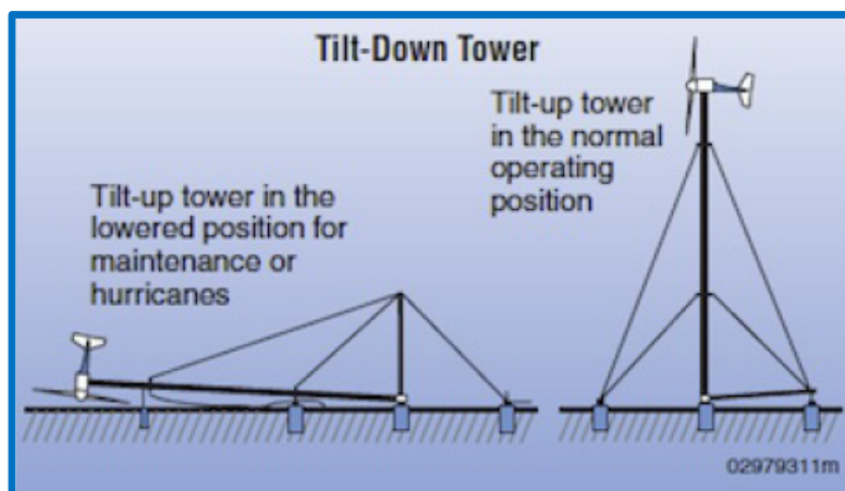
Figure 5. Tilt-Down Tower
