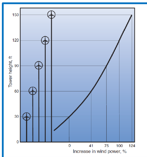
Figure 11. Wind Speeds Increase with Height
